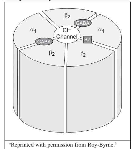
Figure 1. GABA-Benzodiazepine (BZ) Receptor Complex 2
