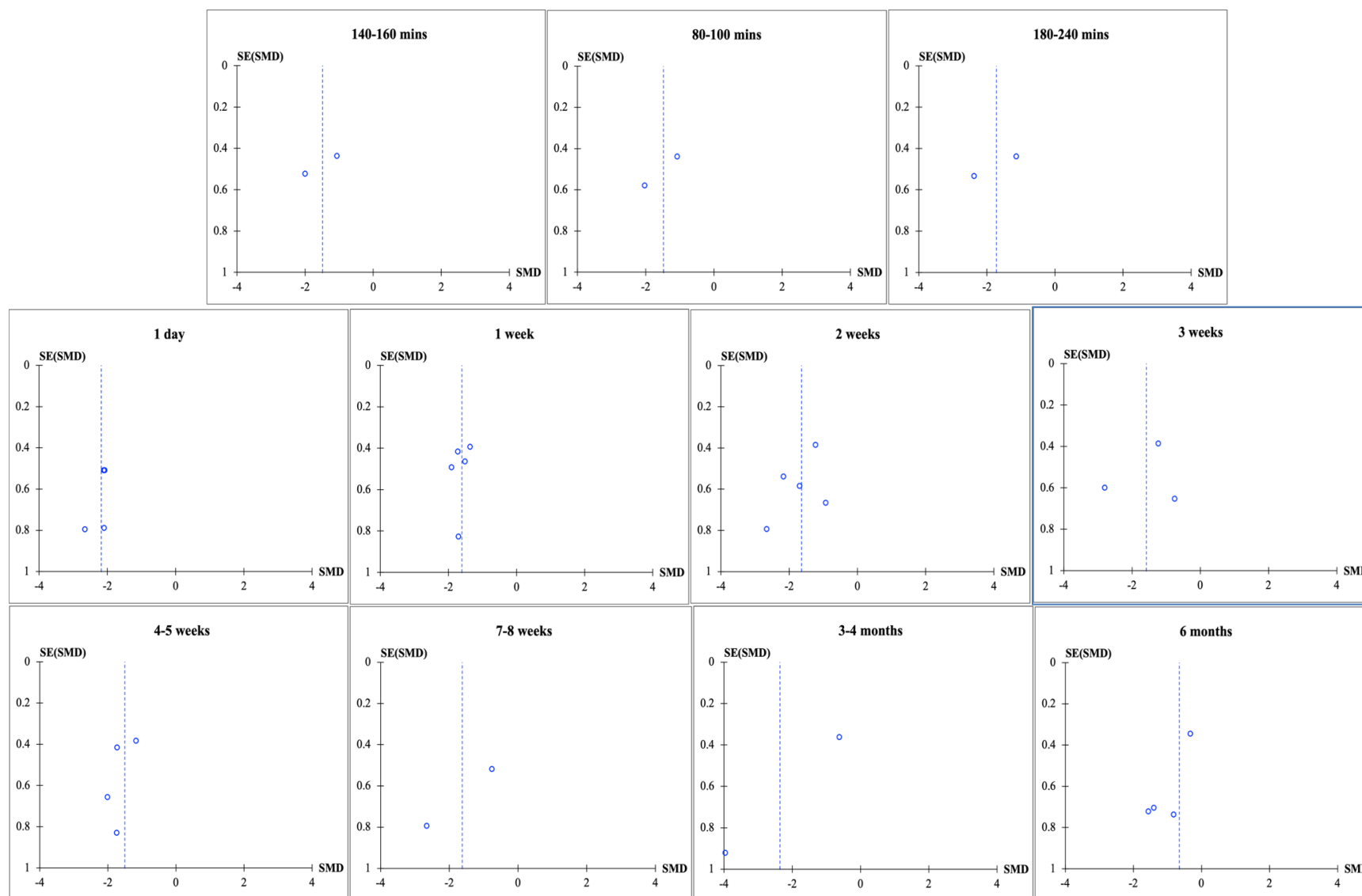
Supplementary Figure 1. Funnel plots
